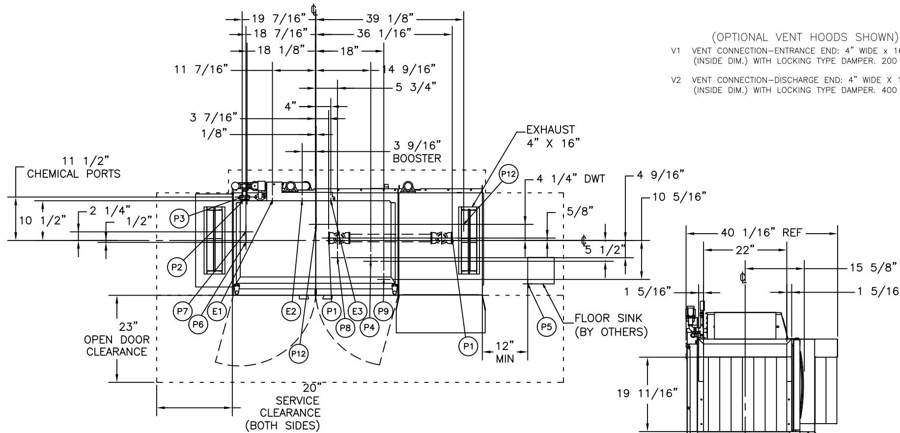
VIEW D-D
