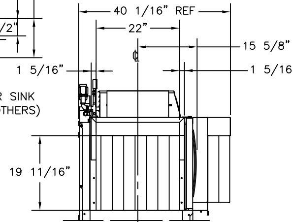
VIEW D-D
